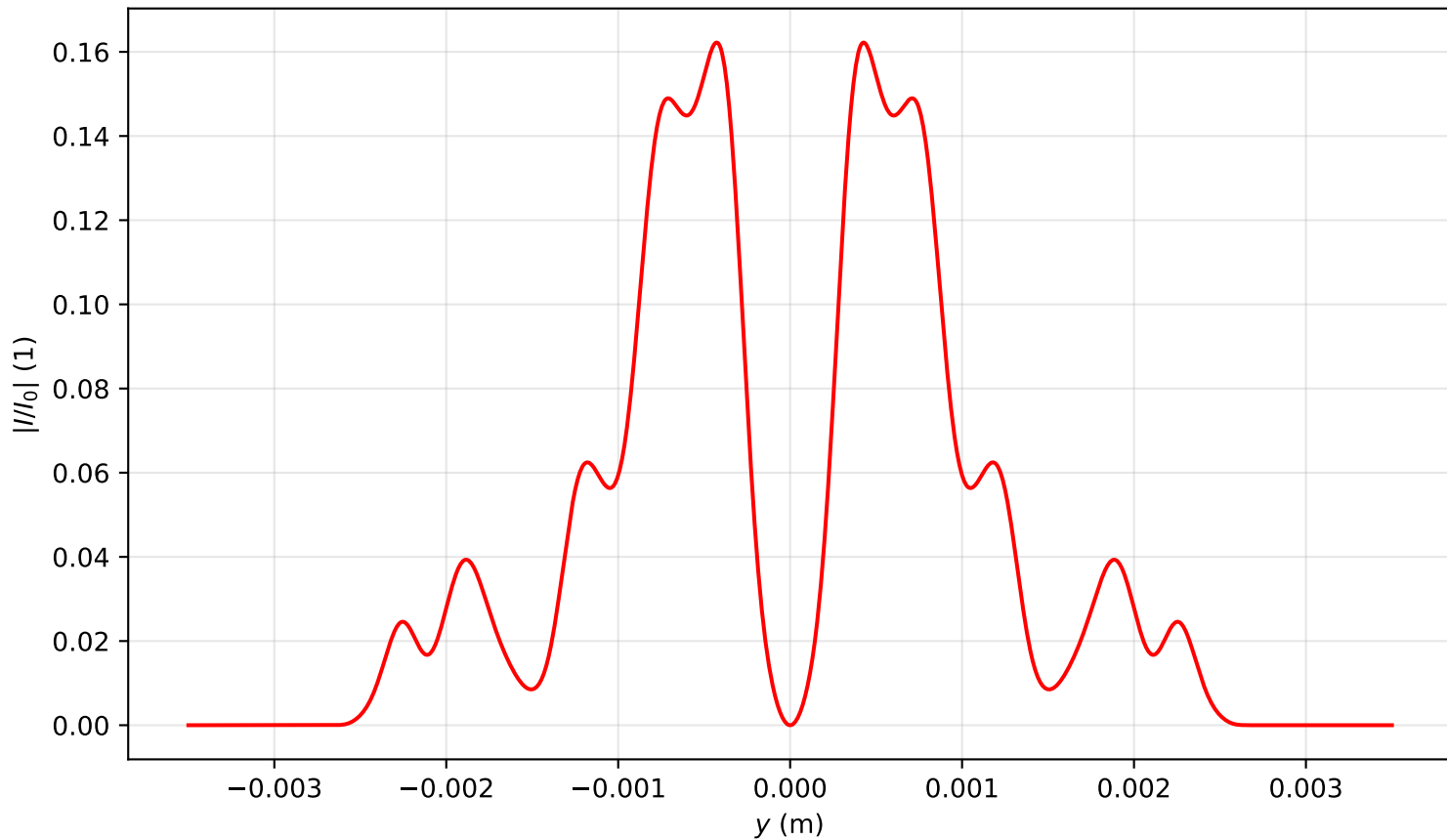
Intensity profile I(x=0, y, z=3.344)/I_0 , \text{Pin}=9.0\text{Pcr} , artificial time
